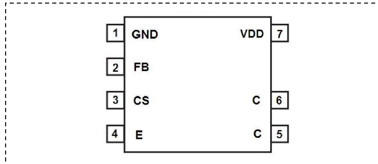
Pin Configuration: TP102 Series ( SOP7 )
