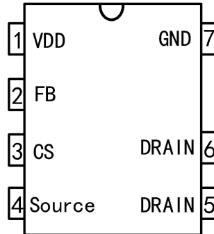
Pin Configuration: G1588P Series
